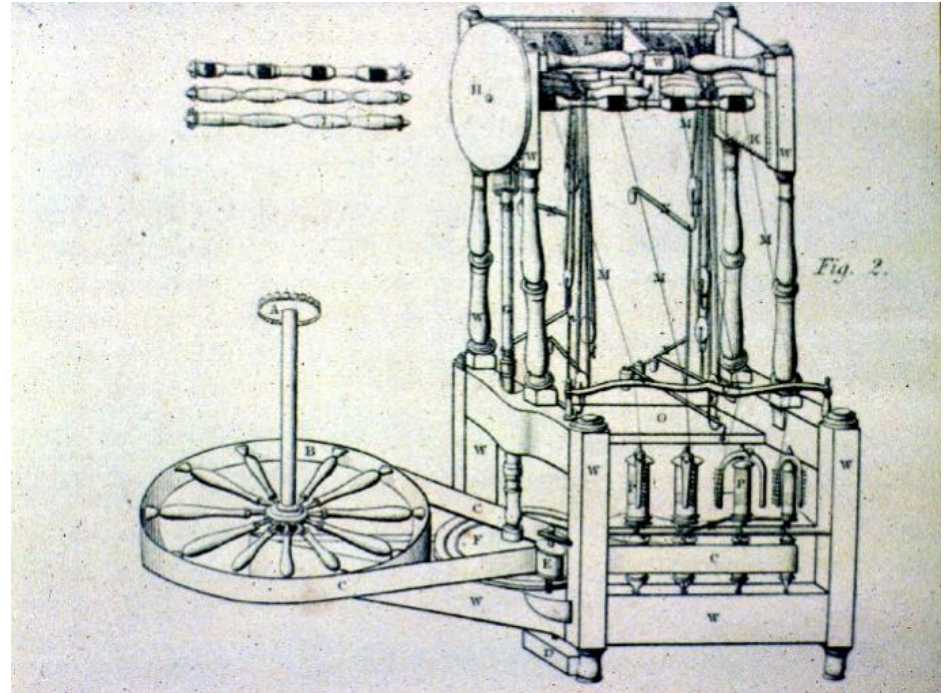
Water-frame (1768)
